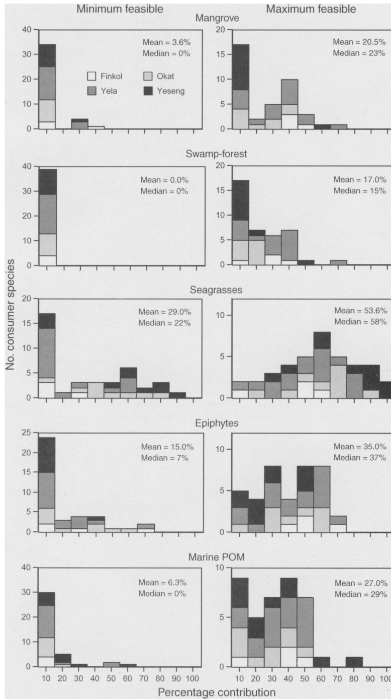
FIG. 2. Histograms of minimum and maximum feasible contributions of five organic matter sources to consumer species in the four estuaries, Kosrae, Federated States of Micronesia, September–December 2000.
